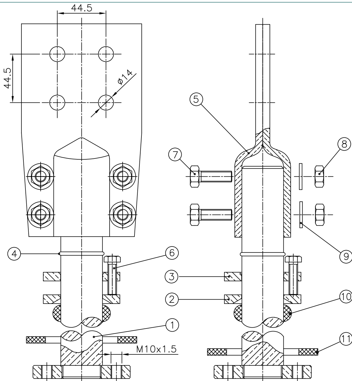
3.4.53.00465 (AE 500060) TERMINAL 1,3KV / 2000 A CONF. NORMA ABNT NBR 16856
